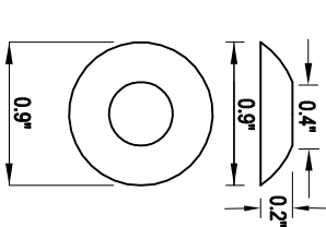
TRUNCATED DOME DETAIL
